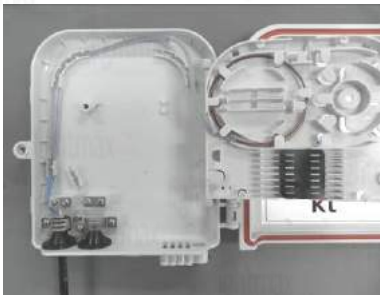
Fibres of the service cable inserted in the protective tuber
