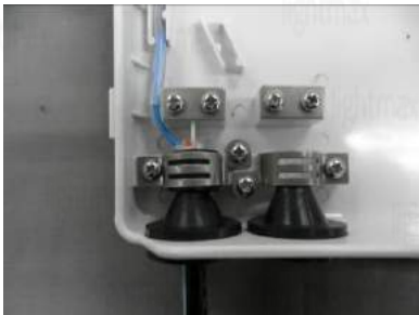
Feeder cable fixation clamps
