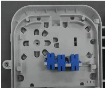
With SC Simplex adapters installed
