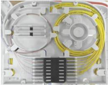
Fusion (or mechanical) splices in the tray
